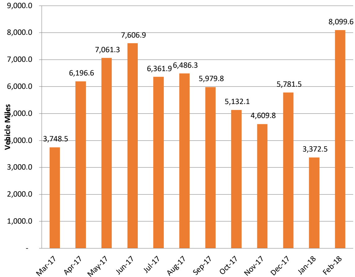
Mean Miles Bet. Road Calls
