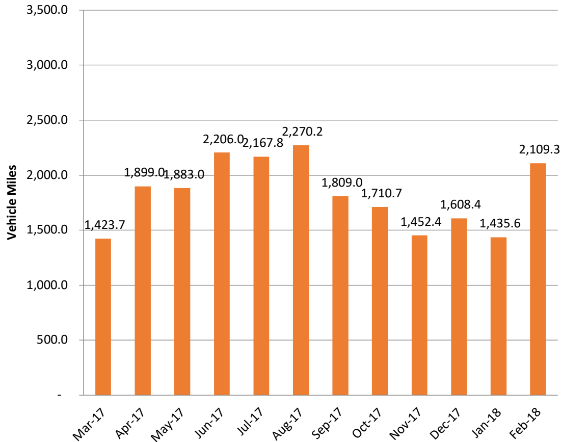
Mean Miles Bet. Mechanical Failures
